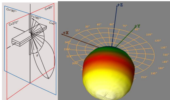
Luminaire light distribution of the 3D
