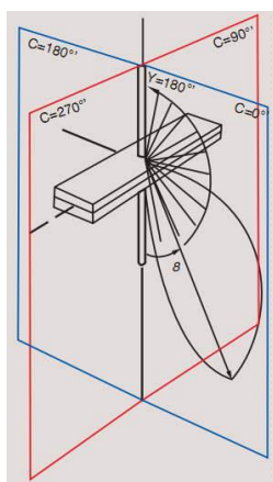
Luminaire light distribution of the 3D
